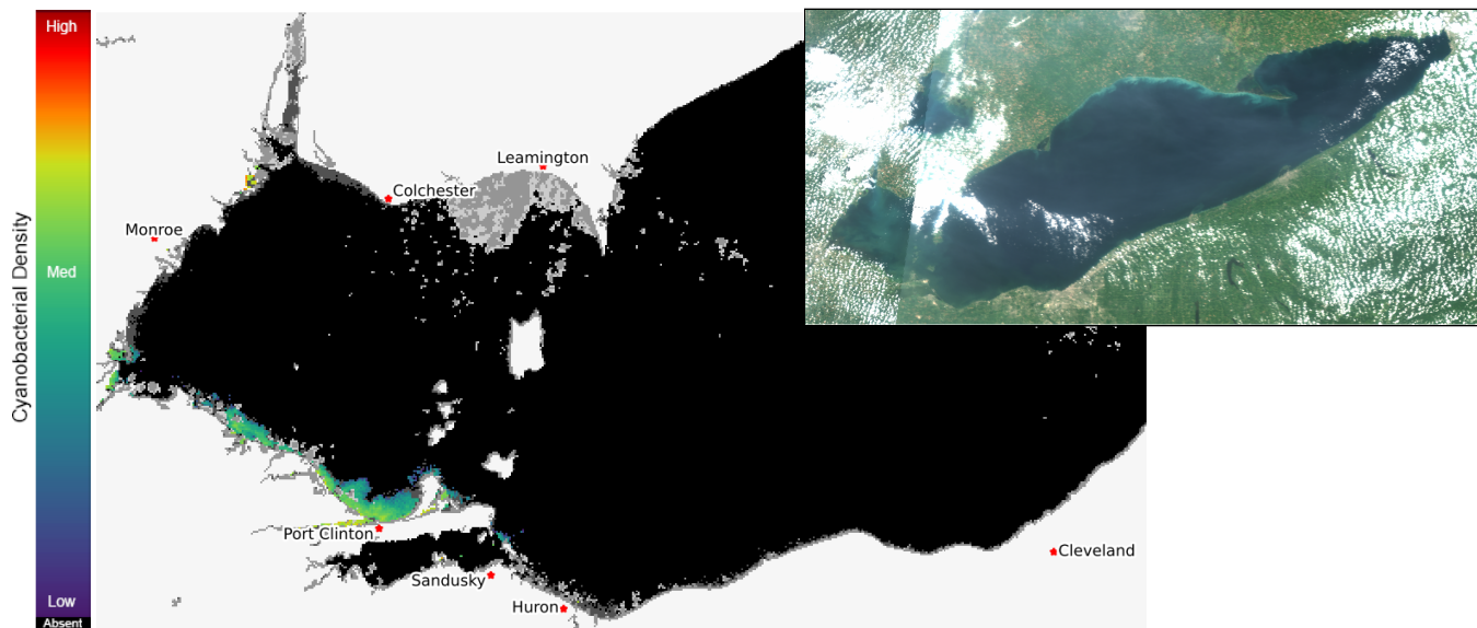
Current Lake Erie Sentinel-3 A and B composited satellite imagery from the Ocean and Land Color Imager (OLCI) on Jul 31, 2021, showing bloom location and extent in the western basin. Grey indicates clouds or missing data. The estimated threshold of cyanobacteria detection is 20,000 cells/mL. Inset shows a truecolor composite image of the entire lake. Data derived from Copernicus Sentinel-3.
