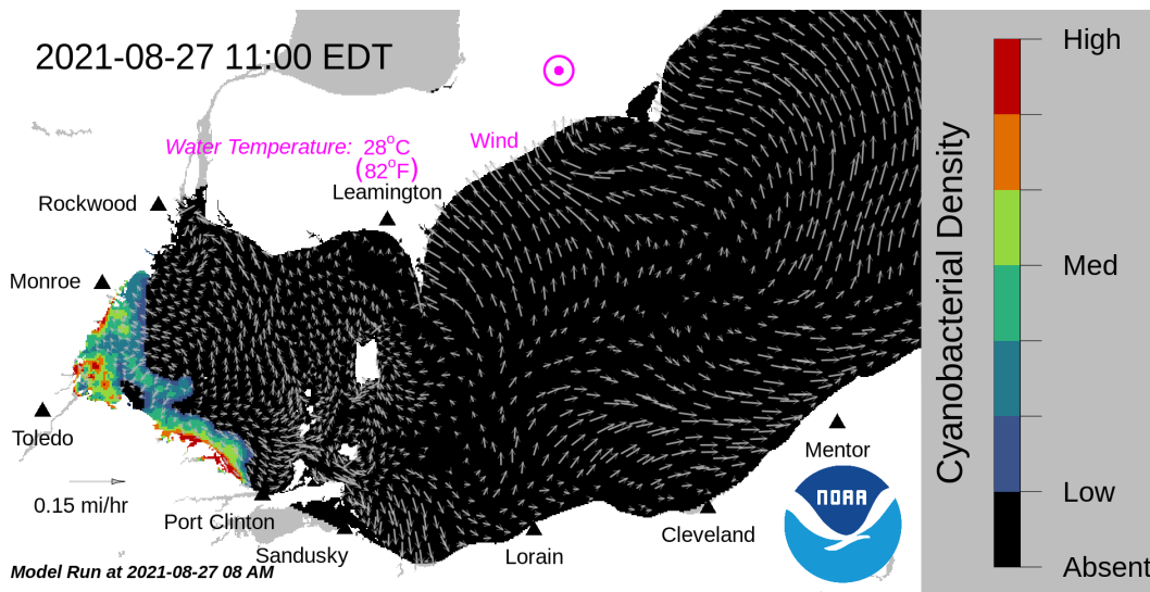
Forecast surface bloom position for Aug 27, modeled from the last satellite image with water currents estimated from the Lake Erie Operational Forecast System (LEOFS). Potential for bloom movement is forecast in 3-dimensions with a hydrodynamic model using satellite imagery and currents. The modeled output does not contain clouds. Black indicates the absence of chlorophyll and gray indicates area with no data. The arrows show forecasted currents. Water temperature and winds (in magenta) are the averages for the western basin from the model.
