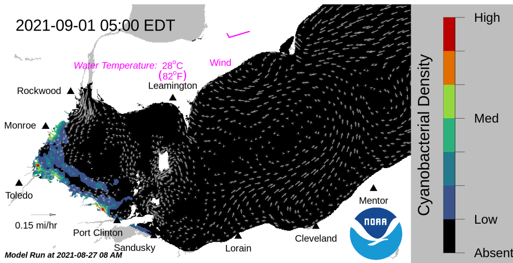
Forecast surface bloom position for Sep 01. Black indicates the absence of chlorophyll and gray indicates area with no data. The arrows show forecasted currents. Water temperature and winds (in magenta) are the averages for the western basin from the model.
