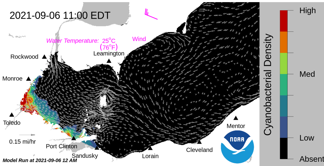
Forecast surface bloom position for Sep 06, modeled from the last satellite image with water currents estimated from the Lake Erie Operational Forecast System (LEOFS). Potential for bloom movement is forecast in 3-dimensions with a hydrodynamic model using satellite imagery and currents. The modeled output does not contain clouds. Black indicates the absence of chlorophyll and gray indicates area with no data. The arrows show forecasted currents. Water temperature and winds (in magenta) are the averages for the western basin from the model.
