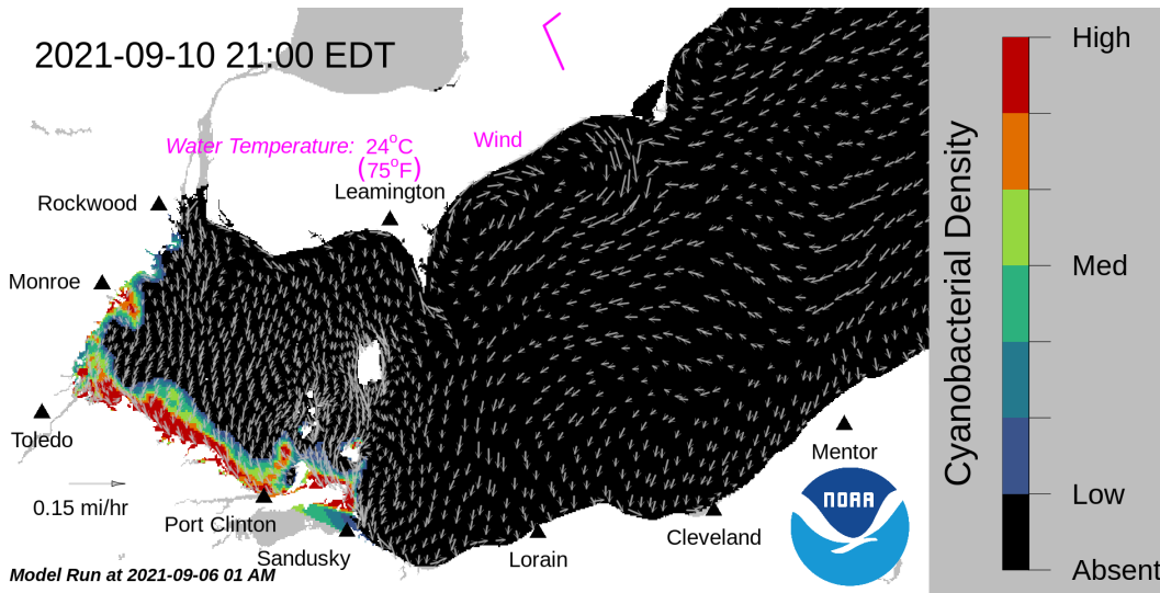
Forecast surface bloom position for Sep 10. Black indicates the absence of chlorophyll and gray indicates area with no data. The arrows show forecasted currents. Water temperature and winds (in magenta) are the averages for the western basin from the model.
