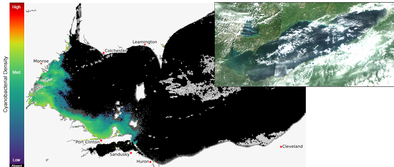
Current Lake Erie Sentinel-3 A and B composited satellite imagery from the Ocean and Land Color Imager (OLCI) on Aug 31, 2021, showing bloom location and extent in the western basin. Grey indicates clouds or missing data. The estimated threshold of cyanobacteria detection is 20,000 cells/mL. Inset shows a truecolor composite image of the entire lake. Data derived from Copernicus Sentinel-3.
