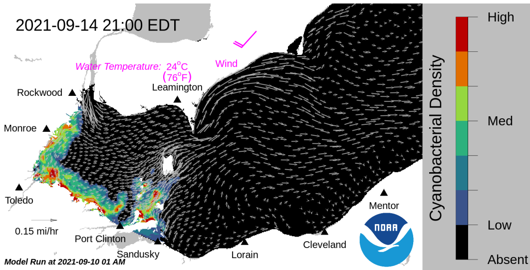
Forecast surface bloom position for Sep 14. Black indicates the absence of chlorophyll and gray indicates area with no data. The arrows show forecasted currents. Water temperature and winds (in magenta) are the averages for the western basin from the model.
