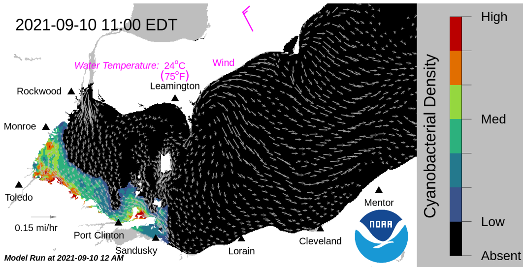
Forecast surface bloom position for Sep 10, modeled from the last satellite image with water currents estimated from the Lake Erie Operational Forecast System (LEOFS). Potential for bloom movement is forecast in 3-dimensions with a hydrodynamic model using satellite imagery and currents. The modeled output does not contain clouds. Black indicates the absence of chlorophyll and gray indicates area with no data. The arrows show forecasted currents. Water temperature and winds (in magenta) are the averages for the western basin from the model.
