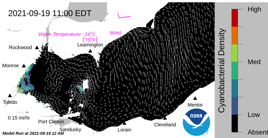
Forecast surface bloom position for Sep 19, modeled from the last satellite image with water currents estimated from the Lake Erie Operational Forecast System (LEOFS). Potential for bloom movement is forecast in 3-dimensions with a hydrodynamic model using satellite imagery and currents. The modeled output does not contain clouds. Black indicates the absence of chlorophyll and gray indicates area with no data. The arrows show forecasted currents. Water temperature and winds (in magenta) are the averages for the western basin from the model.
