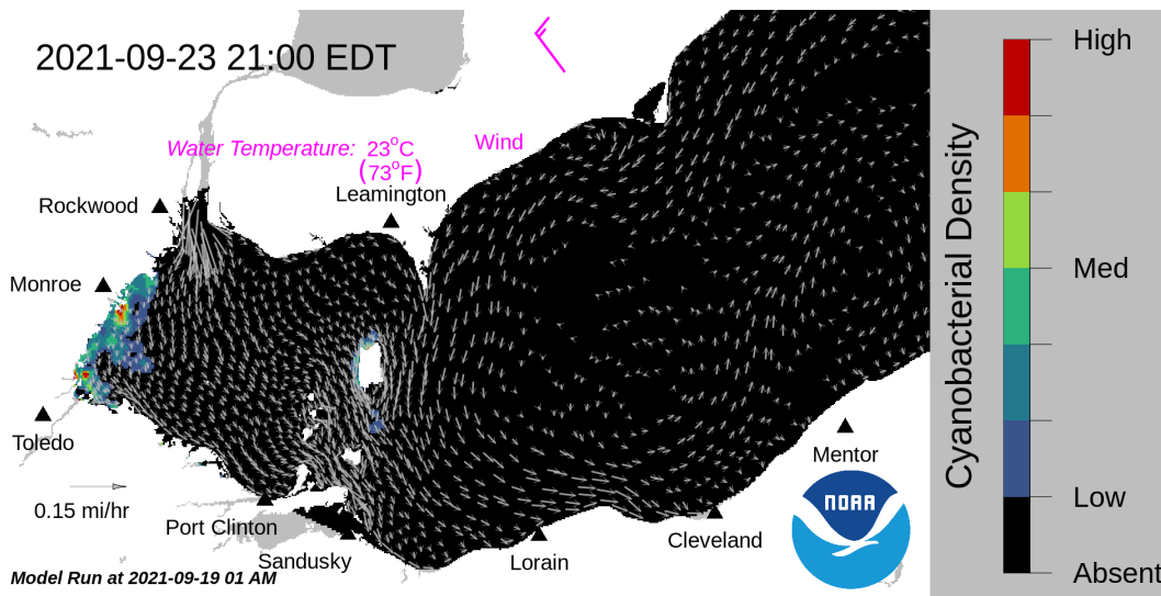
Forecast surface bloom position for Sep 23. Black indicates the absence of chlorophyll and gray indicates area with no data. The arrows show forecasted currents. Water temperature and winds (in magenta) are the averages for the western basin from the model.
