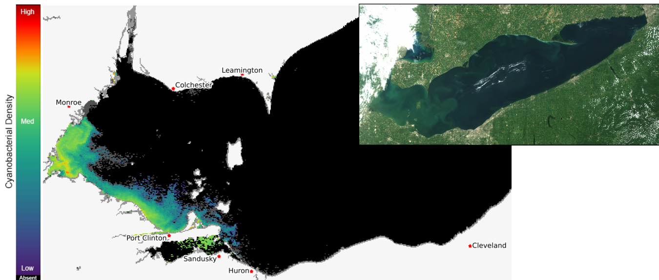
Current Lake Erie Sentinel-3A satellite imagery from the Ocean and Land Color Imager (OLCI) on Aug 24, 2021, showing bloom location and extent in the western basin. Grey indicates clouds or missing data. The estimated threshold of cyanobacteria detection is 20,000 cells/mL. Inset shows a truecolor image of the entire lake. Data derived from Copernicus Sentinel-3.
