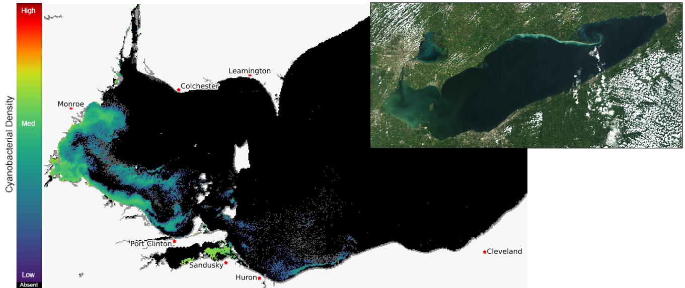
Current Lake Erie Sentinel-3 satellite imagery from the Ocean and Land Color Imager (OLCI) on Sep 05, 2023, showing bloom location and extent in the western basin. Grey indicates clouds or missing data. The estimated threshold of cyanobacteria detection is 20,000 cells/mL. Inset shows a truecolor image of the entire lake. Data derived from Copernicus Sentinel-3.
