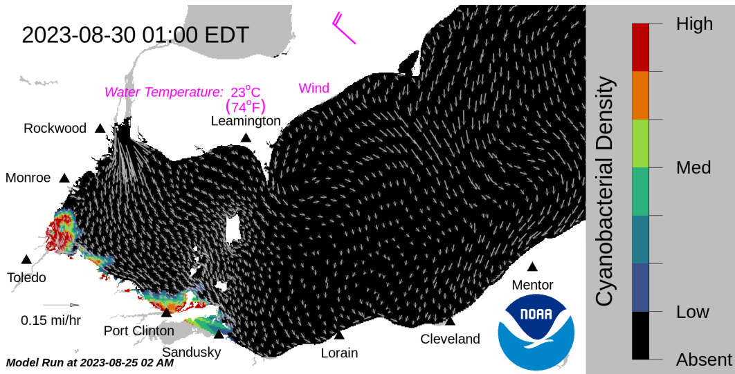
Forecast surface bloom position for Aug 30. Black indicates the absence of chlorophyll and gray indicates area with no data. The arrows show forecasted currents. Water temperature and winds (in magenta) are the averages for the western basin from the model.
