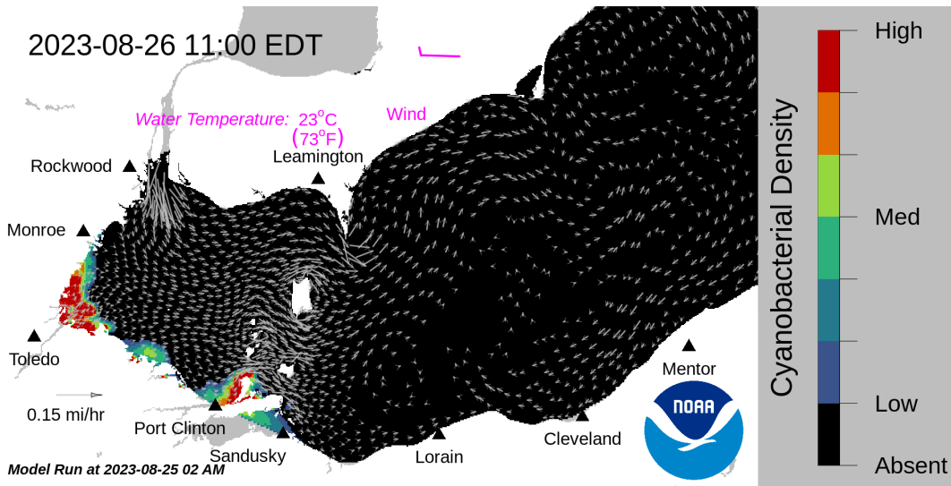
Forecast surface bloom position for Aug 26, modeled from the last satellite image with water currents estimated from the Lake Erie Operational Forecast System (LEOFS). Potential for bloom movement is forecast in 3-dimensions with a hydrodynamic model using satellite imagery and currents. The modeled output does not contain clouds. Black indicates the absence of chlorophyll and gray indicates area with no data. The arrows show forecasted currents. Water temperature and winds (in magenta) are the averages for the western basin from the model.
