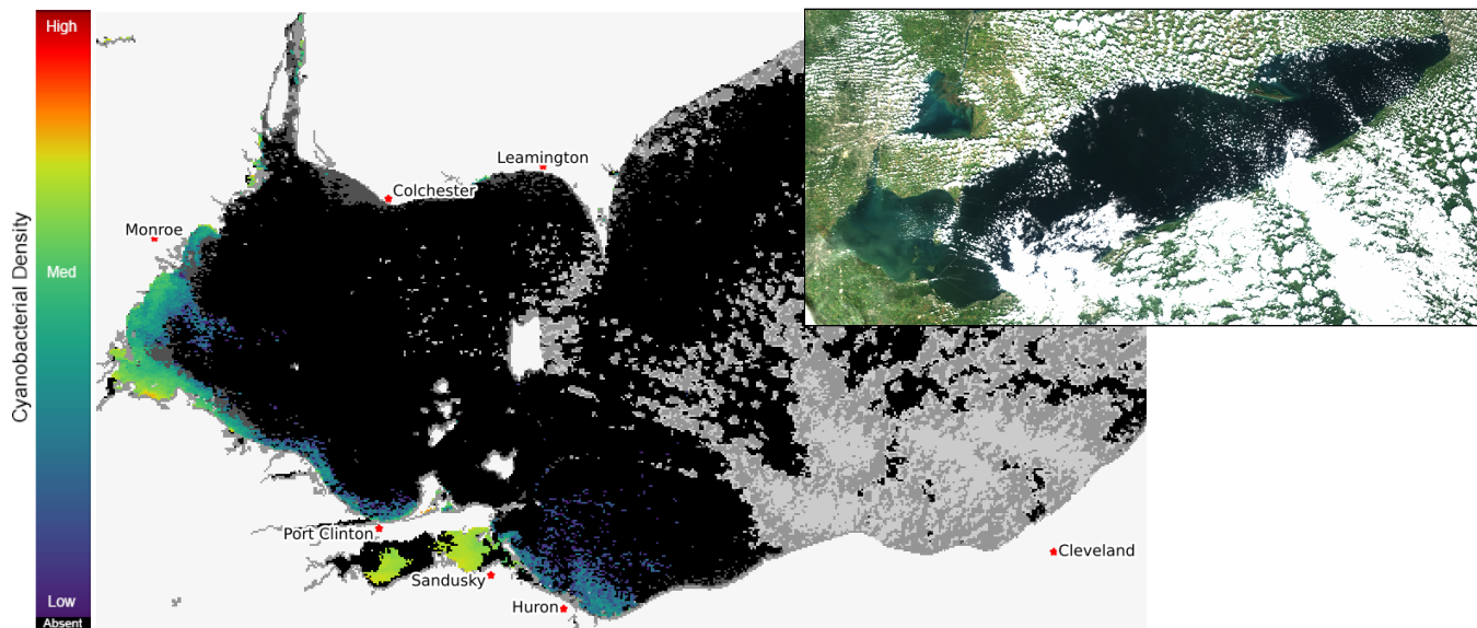
Current Lake Erie Sentinel-3 satellite imagery from the Ocean and Land Color Imager (OLCI) on Sep 19, 2023, showing bloom location and extent in the western basin. Grey indicates clouds or missing data. The estimated threshold of cyanobacteria detection is 20,000 cells/mL. Inset shows a truecolor image of the entire lake. Data derived from Copernicus Sentinel-3.
