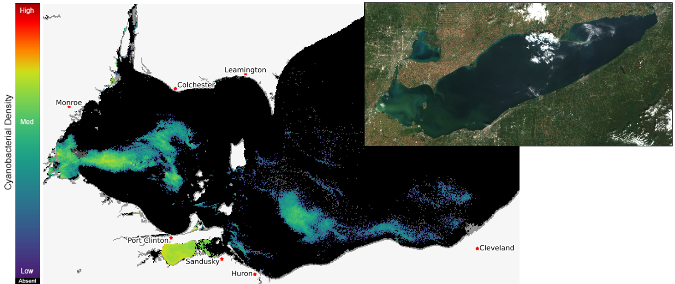
Current Lake Erie Sentinel-3 satellite imagery from the Ocean and Land Color Imager (OLCI) on Oct 02, 2023, showing bloom location and extent in the western basin. Grey indicates clouds or missing data. The estimated threshold of cyanobacteria detection is 20,000 cells/mL. Inset shows a truecolor image of the entire lake. Data derived from Copernicus Sentinel-3.
