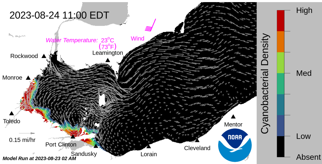
Forecast surface bloom position for Aug 24, modeled from the last satellite image with water currents estimated from the Lake Erie Operational Forecast System (LEOFS). Potential for bloom movement is forecast in 3-dimensions with a hydrodynamic model using satellite imagery and currents. The modeled output does not contain clouds. Black indicates the absence of chlorophyll and gray indicates area with no data. The arrows show forecasted currents. Water temperature and winds (in magenta) are the averages for the western basin from the model.
