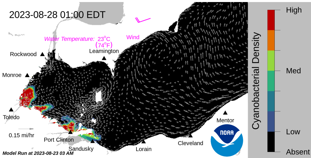
Forecast surface bloom position for Aug 28. Black indicates the absence of chlorophyll and gray indicates area with no data. The arrows show forecasted currents. Water temperature and winds (in magenta) are the averages for the western basin from the model.
