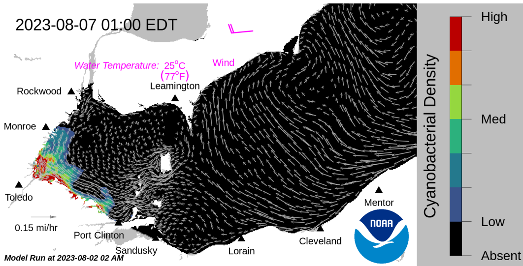
Forecast surface bloom position for Aug 07. Black indicates the absence of chlorophyll and gray indicates area with no data. The arrows show forecasted currents. Water temperature and winds (in magenta) are the averages for the western basin from the model.
