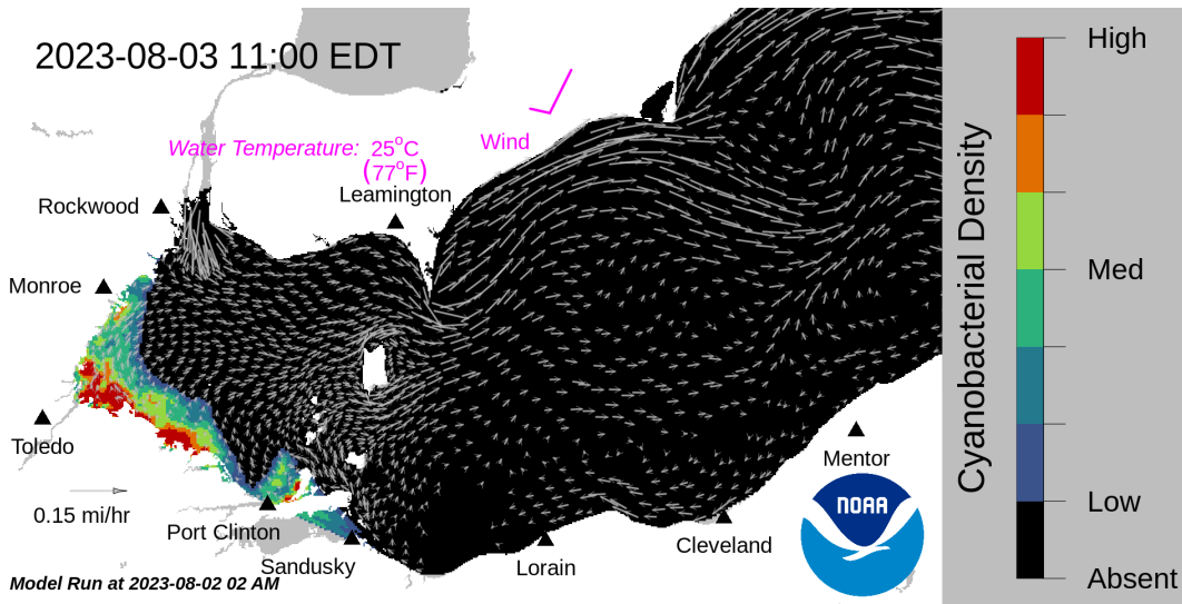
Forecast surface bloom position for Aug 03, modeled from the last satellite image with water currents estimated from the Lake Erie Operational Forecast System (LEOFS). Potential for bloom movement is forecast in 3-dimensions with a hydrodynamic model using satellite imagery and currents. The modeled output does not contain clouds. Black indicates the absence of chlorophyll and gray indicates area with no data. The arrows show forecasted currents. Water temperature and winds (in magenta) are the averages for the western basin from the model.
