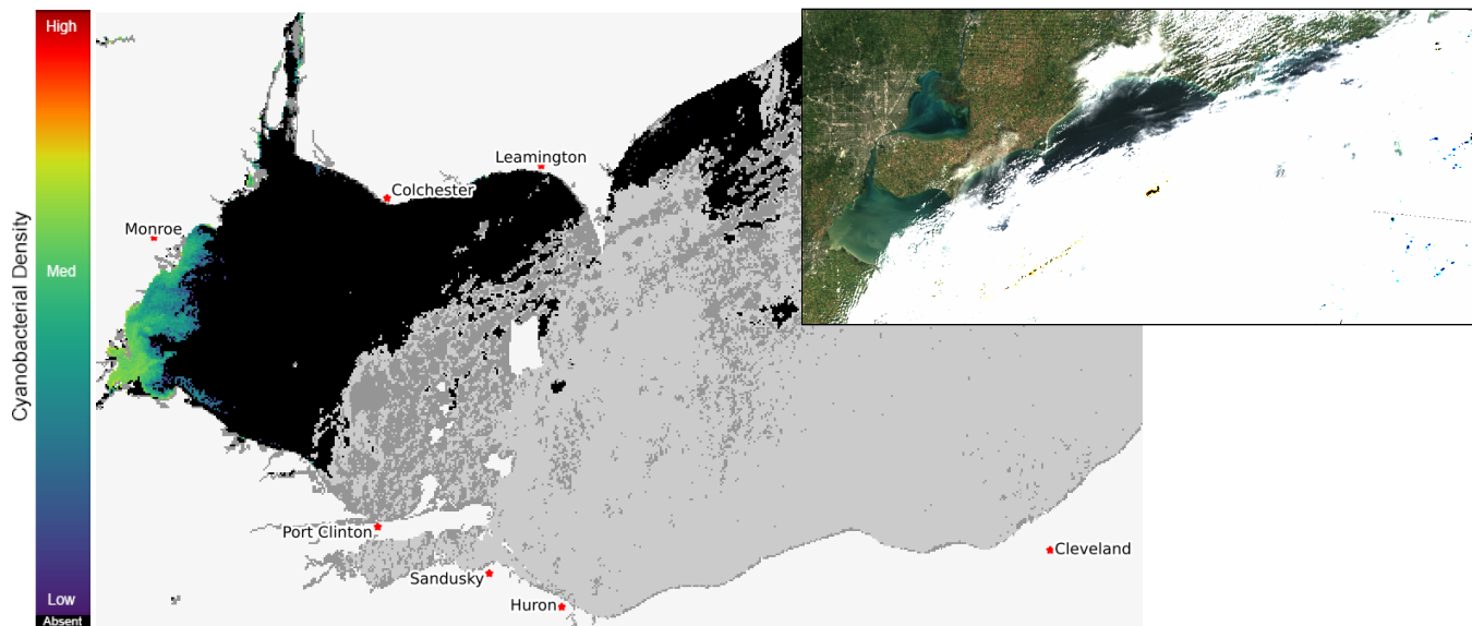
Current Lake Erie Sentinel-3 satellite imagery from the Ocean and Land Color Imager (OLCI) on Sep 24, 2023, showing bloom location and extent in the western basin. Grey indicates clouds or missing data. The estimated threshold of cyanobacteria detection is 20,000 cells/mL. Inset shows a truecolor image of the entire lake. Data derived from Copernicus Sentinel-3.
