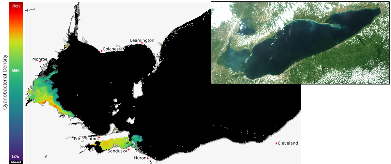
Current Lake Erie Sentinel-3 satellite imagery from the Ocean and Land Color Imager (OLCI) on Jul 14, 2023, showing bloom location and extent in the western basin. Grey indicates clouds or missing data. The estimated threshold of cyanobacteria detection is 20,000 cells/mL. Inset shows a truecolor image of the entire lake. Data derived from Copernicus Sentinel-3.
