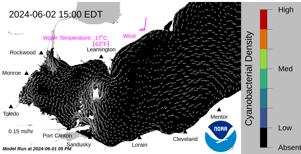
Forecast surface bloom position for Jun 02, modeled from the last satellite image with water currents estimated from the Lake Erie Operational Forecast System (LEOFS). Potential for bloom movement is forecast in 3-dimensions with a hydrodynamic model using satellite imagery and currents. The modeled output does not contain clouds. Black indicates the absence of chlorophyll and gray indicates area with no data. The arrows show forecasted currents. Water temperature and winds (in magenta) are the averages for the western basin from the model.
