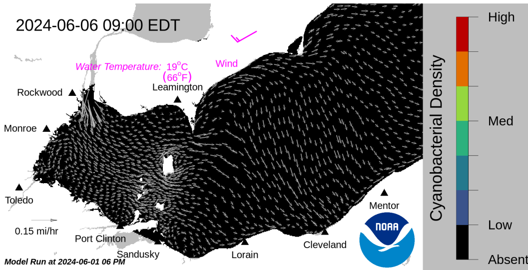
Forecast surface bloom position for Jun 06. Black indicates the absence of chlorophyll and gray indicates area with no data. The arrows show forecasted currents. Water temperature and winds (in magenta) are the averages for the western basin from the model.
