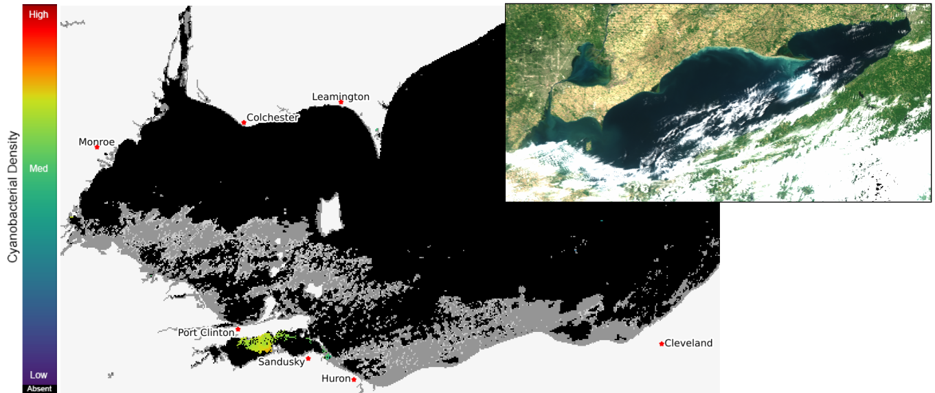
Current Lake Erie Sentinel-3 satellite imagery from the Ocean and Land Color Imager (OLCI) on Jun 14, 2024, showing bloom location and extent in the western basin. Grey indicates clouds or missing data. The estimated threshold of cyanobacteria detection is 20,000 cells/mL. Inset shows a truecolor image of the entire lake. Data derived from Copernicus Sentinel-3.
