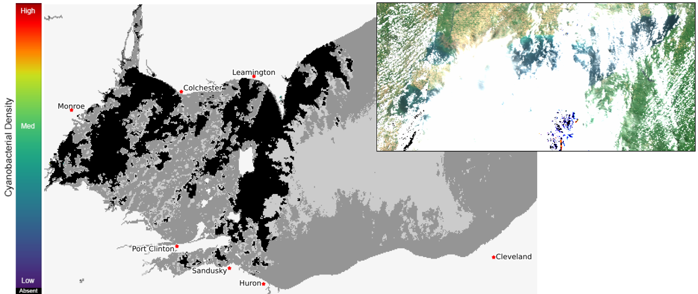
Current Lake Erie Sentinel-3 satellite imagery from the Ocean and Land Color Imager (OLCI) on May 22, 2024, showing bloom location and extent in the western basin. Grey indicates clouds or missing data. The estimated threshold of cyanobacteria detection is 20,000 cells/mL. Inset shows a truecolor image of the entire lake. Data derived from Copernicus Sentinel-3.
