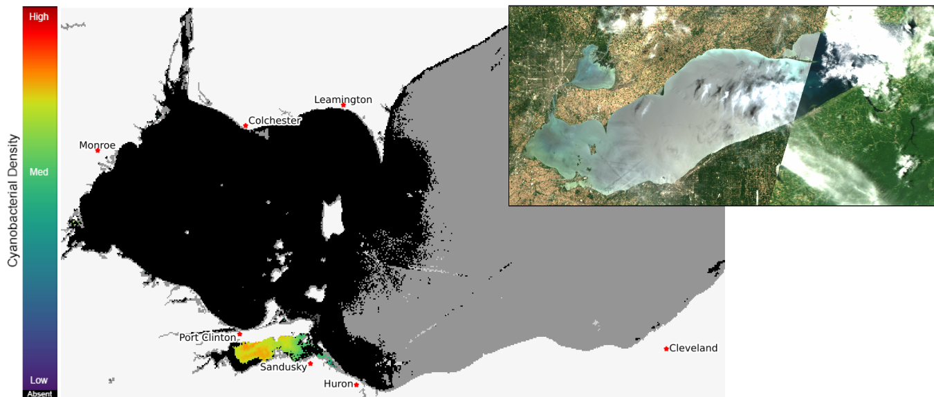
Current Lake Erie Sentinel-3 satellite imagery from the Ocean and Land Color Imager (OLCI) on Jun 16, 2024, showing bloom location and extent in the western basin. Grey indicates clouds or missing data. The estimated threshold of cyanobacteria detection is 20,000 cells/mL. Inset shows a truecolor image of the entire lake. Data derived from Copernicus Sentinel-3.
