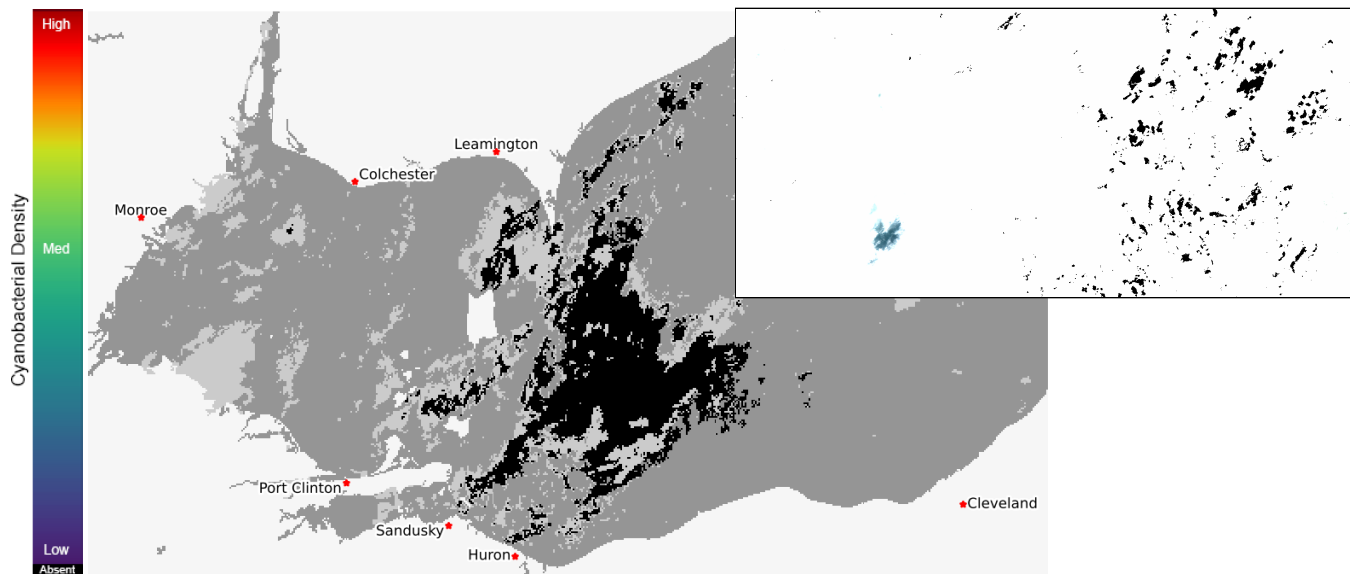
Current Lake Erie Sentinel-3 satellite imagery from the Ocean and Land Color Imager (OLCI) on Jun 02, 2024, showing bloom location and extent in the western basin. Grey indicates clouds or missing data. The estimated threshold of cyanobacteria detection is 20,000 cells/mL. Inset shows a truecolor image of the entire lake. Data derived from Copernicus Sentinel-3.
