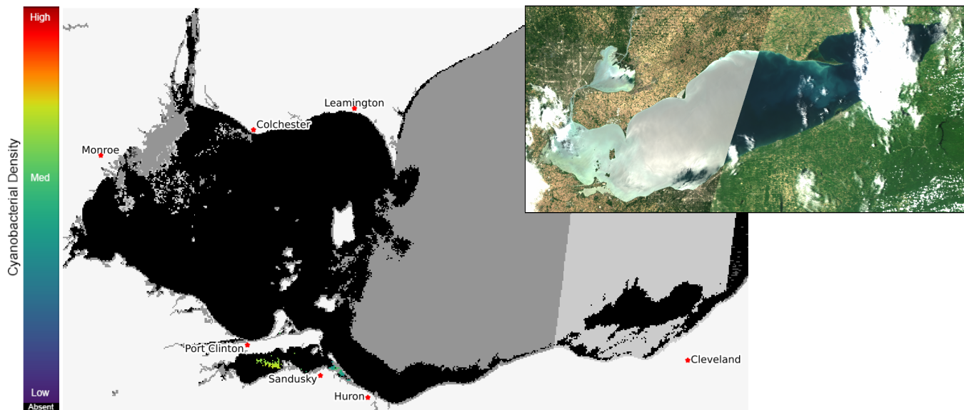
Current Lake Erie Sentinel-3 satellite imagery from the Ocean and Land Color Imager (OLCI) on Jun 12, 2024, showing bloom location and extent in the western basin. Grey indicates clouds or missing data. The estimated threshold of cyanobacteria detection is 20,000 cells/mL. Inset shows a truecolor image of the entire lake. Data derived from Copernicus Sentinel-3.
