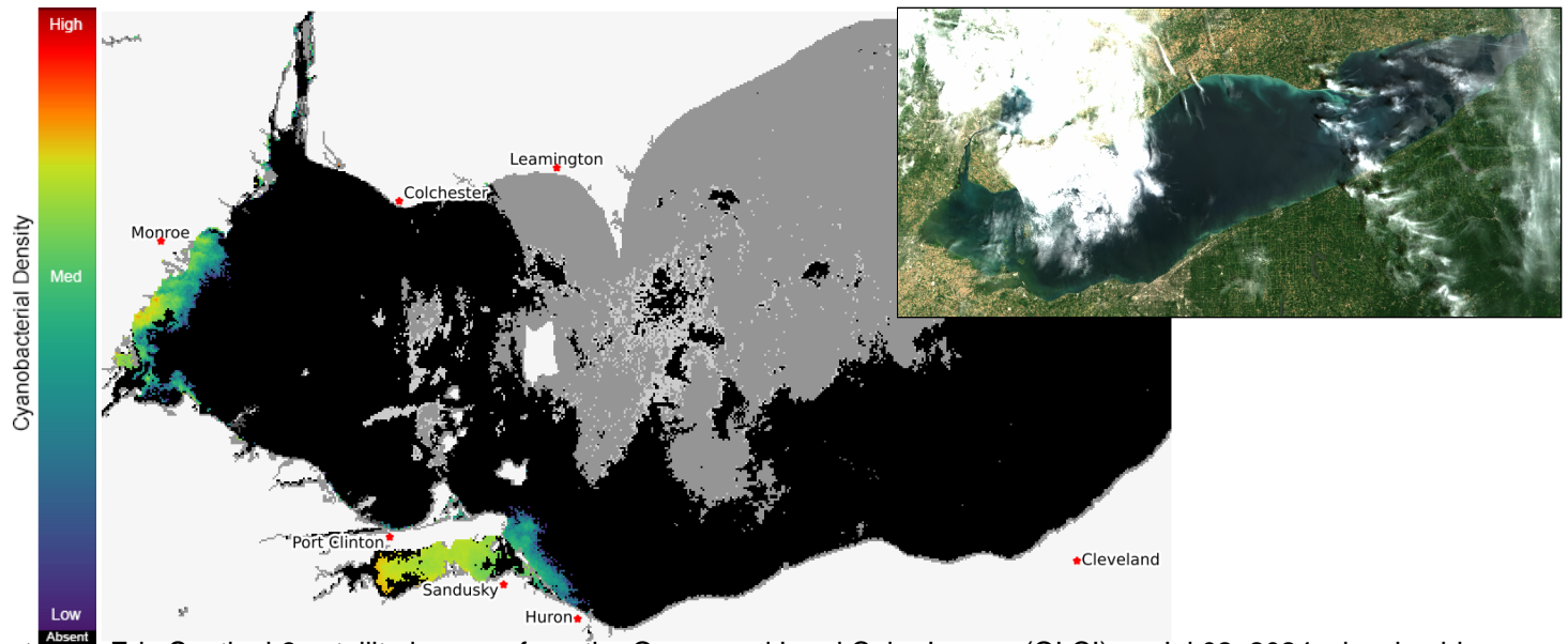
Current Lake Erie Sentinel-3 satellite imagery from the Ocean and Land Color Imager (OLCI) on Jul 02, 2024, showing bloom location and extent in the western basin. Grey indicates clouds or missing data. The estimated threshold of cyanobacteria detection is 20,000 cells/mL. Inset shows a truecolor image of the entire lake. Data derived from Copernicus Sentinel-3.
