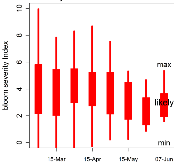
Figure 3: Loading season projections for 2015 starting March 1st, where a bloom severity of 10 indicates the record-breaking bloom of 2011. The event caused by intense rainfall on May 31 caused a slight increase in the projected bloom. Large flow events in the next month could cause an additional increase in the projection.
