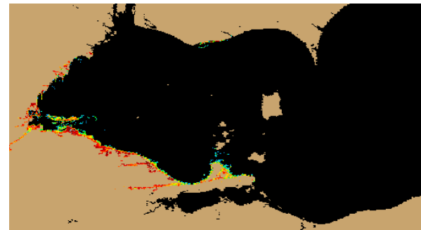
Figure 3. Forecast position of Microcystis spp. for July 03 using GLCFS modeled currents to move the bloom from June 29 image.
