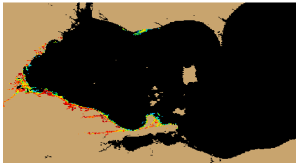
Figure 2. Nowcast position of Microcystis spp. bloom for June 30 using GLCFS modeled currents to move the bloom from the June 29 image.
